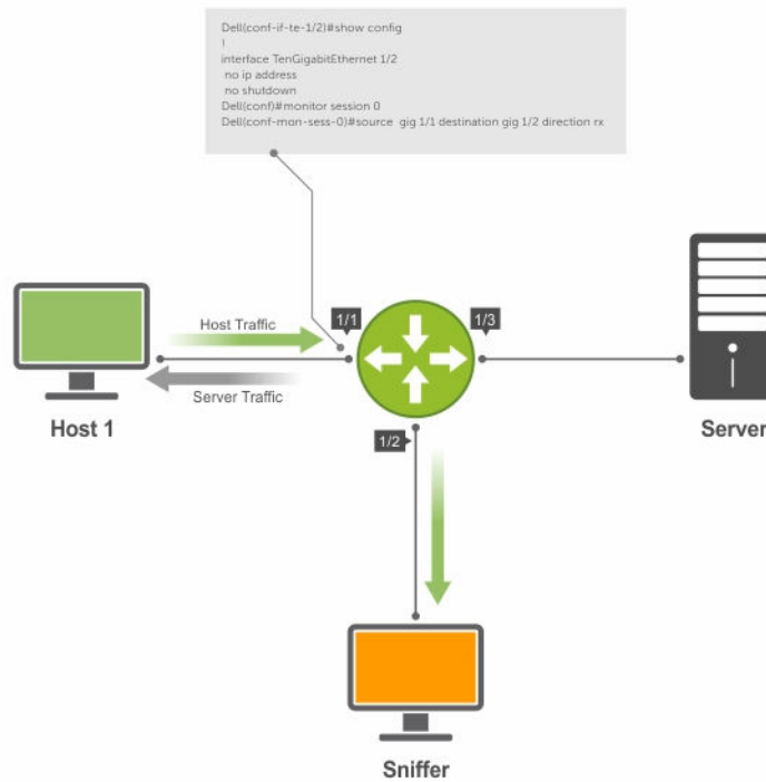
Figure 95. Port Monitoring Example
